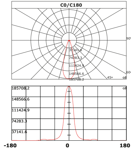
30° Lens
