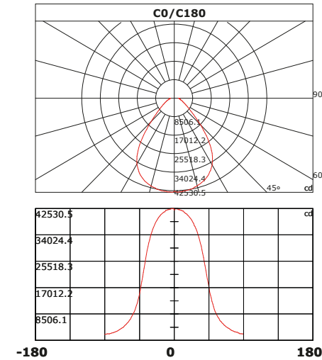
90° Lens
