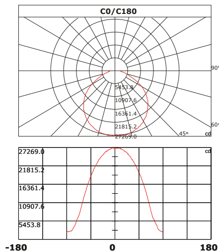
120° Lens
