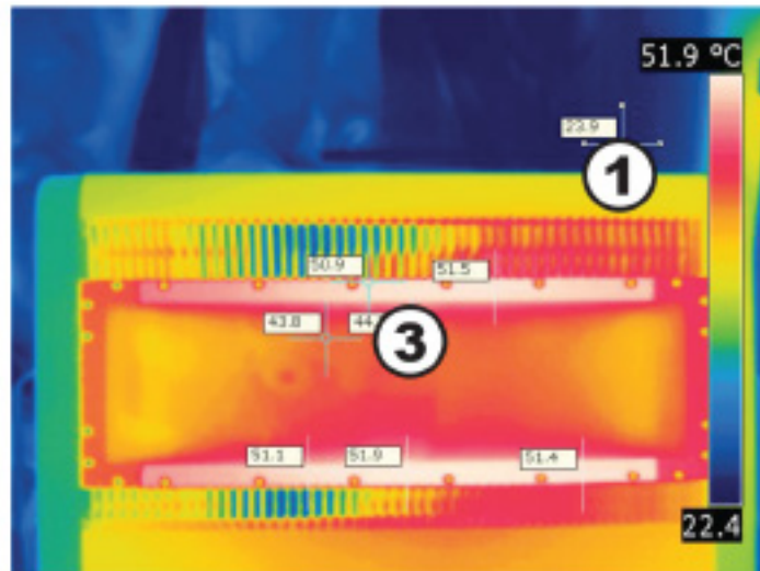
Front Projection
